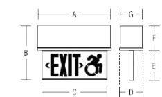
Surface Wall
